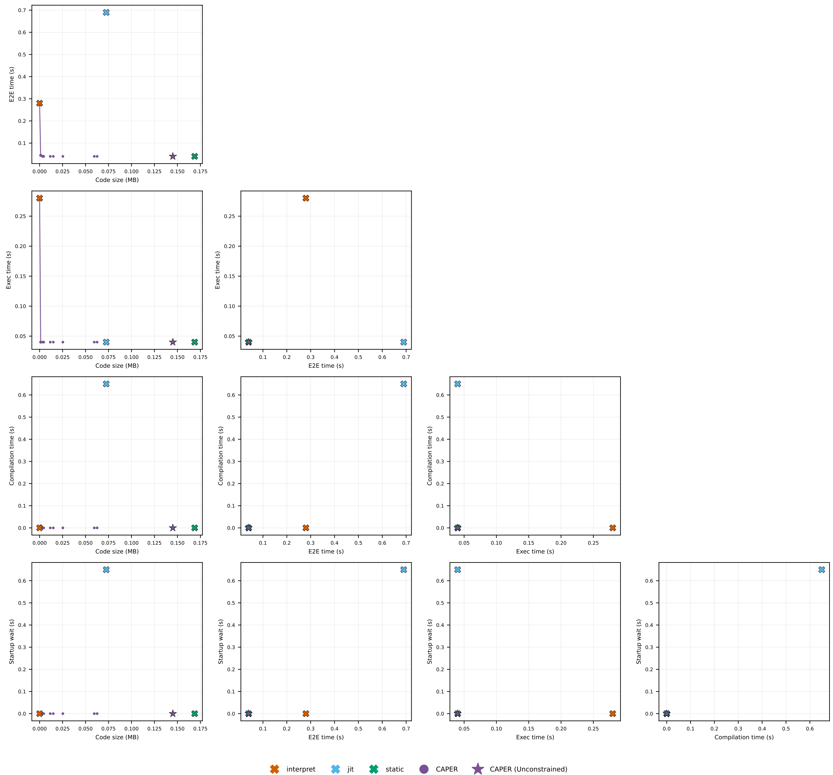
jacobi-1d · jacobi-1d: pairwise metric trade-offs
