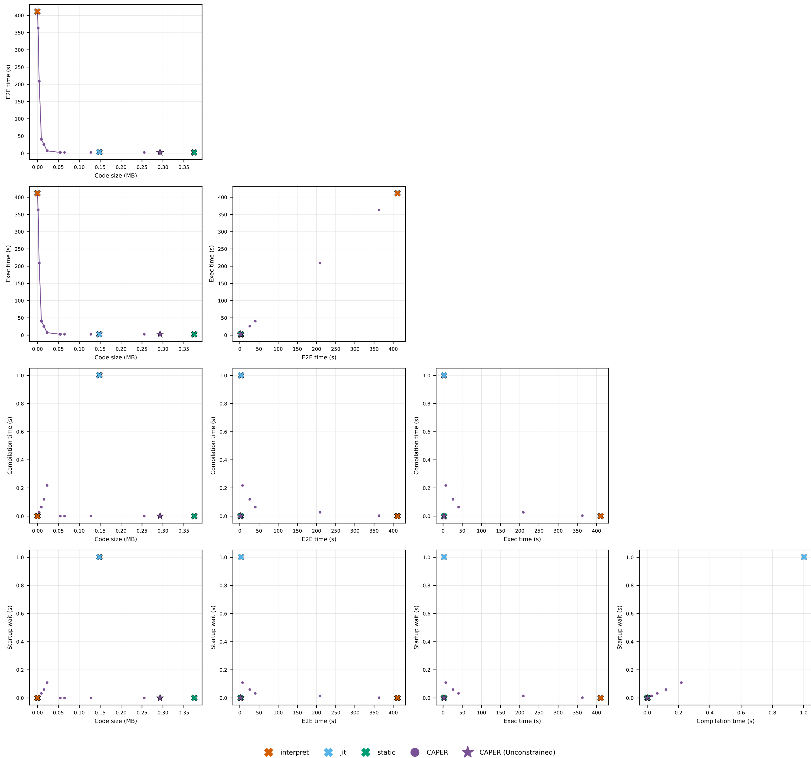
MG · MG: pairwise metric trade-offs
