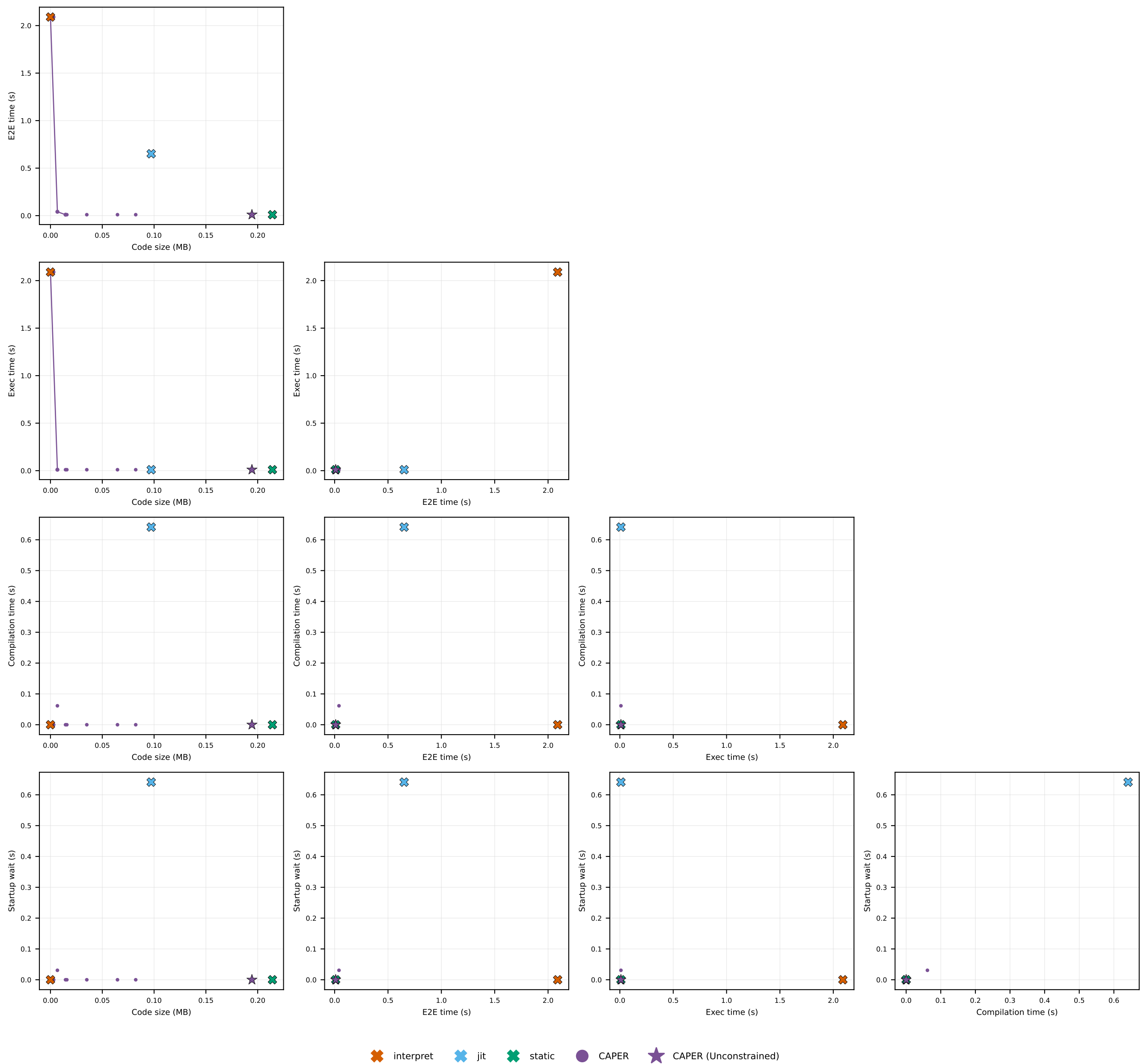
sha · sha: pairwise metric trade-offs
