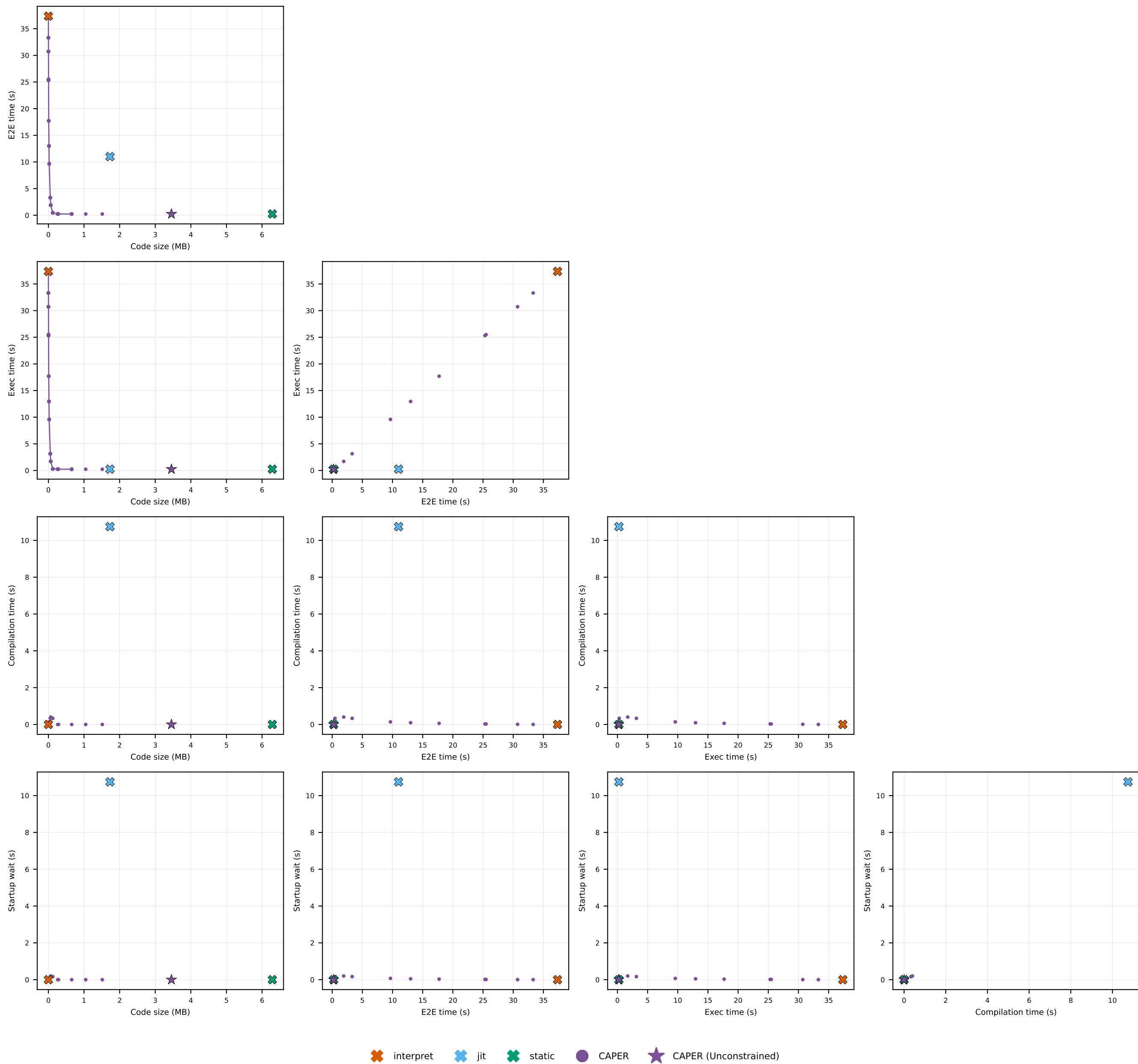
SQLite · bulk-insert-transaction: pairwise metric trade-offs
