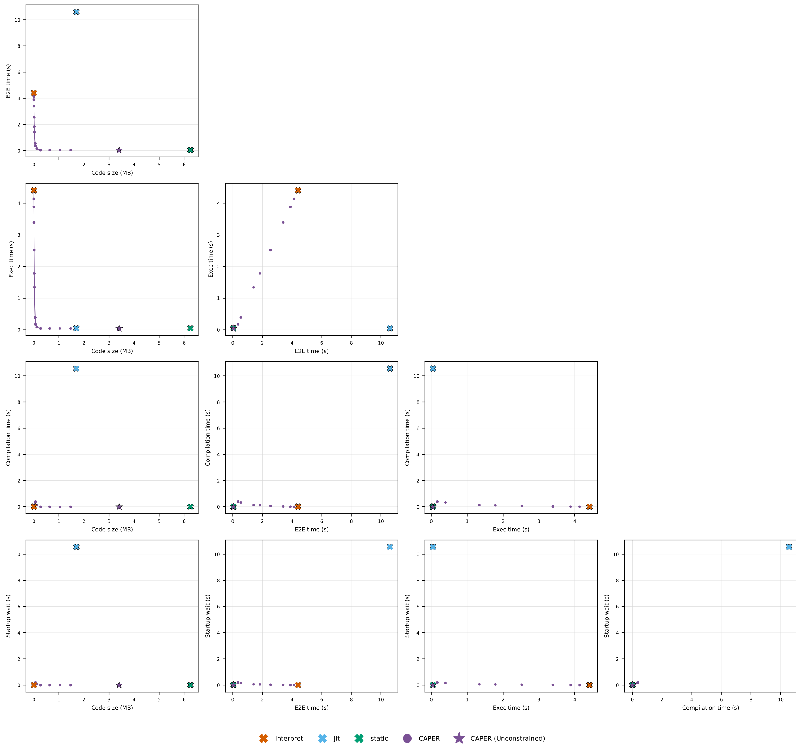
SQLite · create-insert-select: pairwise metric trade-offs
