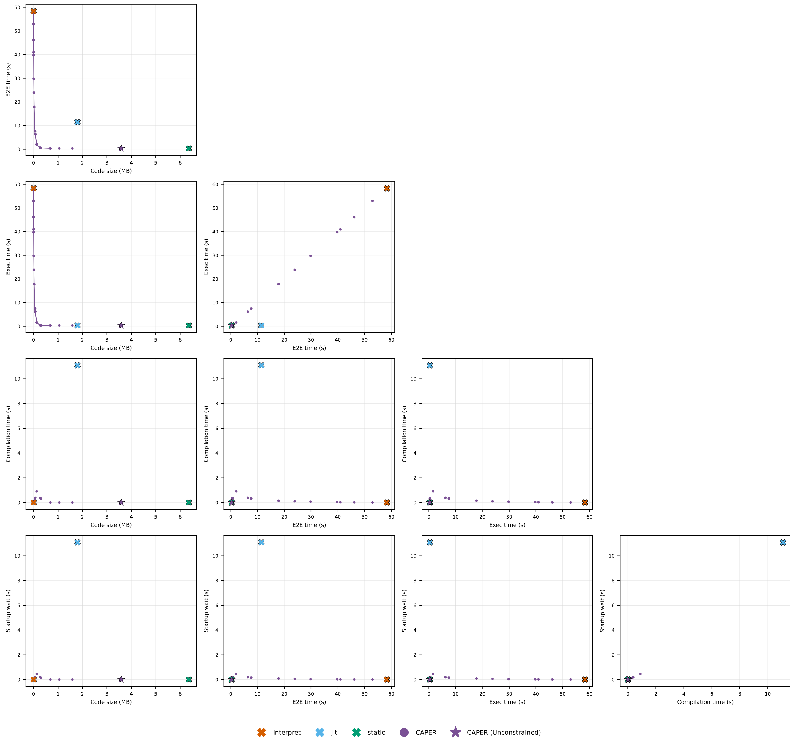
SQLite · group-by-aggregate: pairwise metric trade-offs
