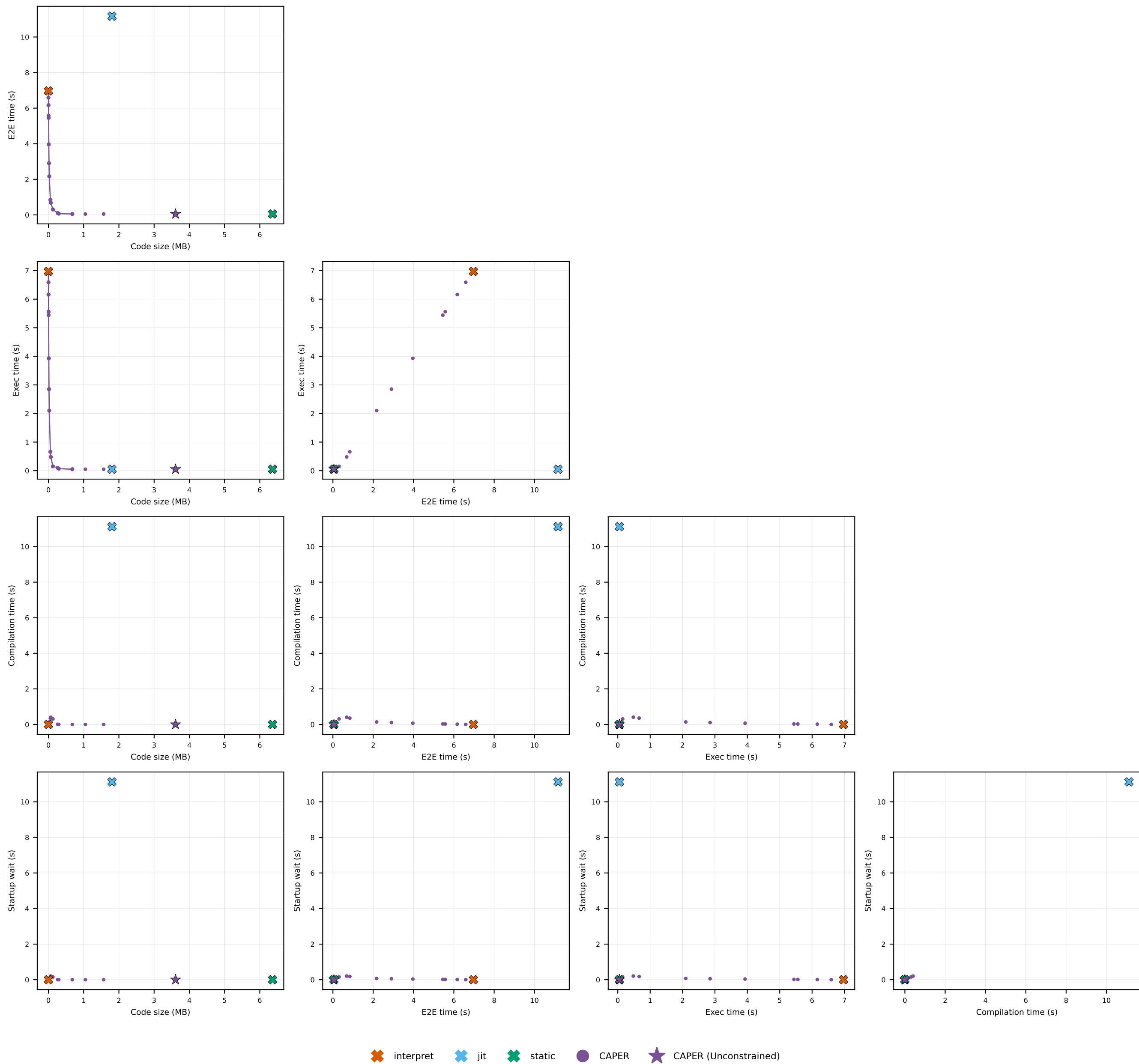
SQLite · multi-table-join: pairwise metric trade-offs
