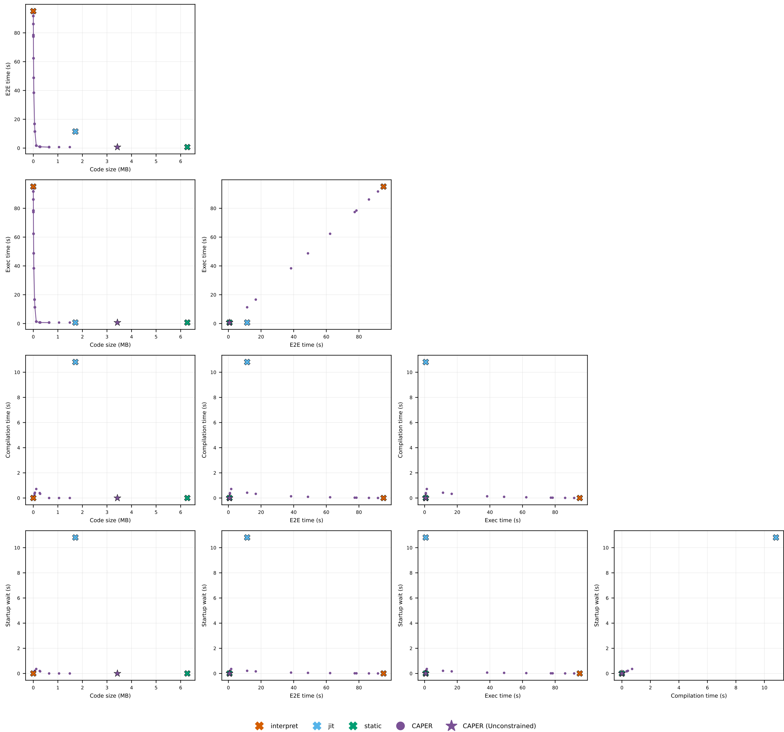
SQLite · order-by-limit: pairwise metric trade-offs
