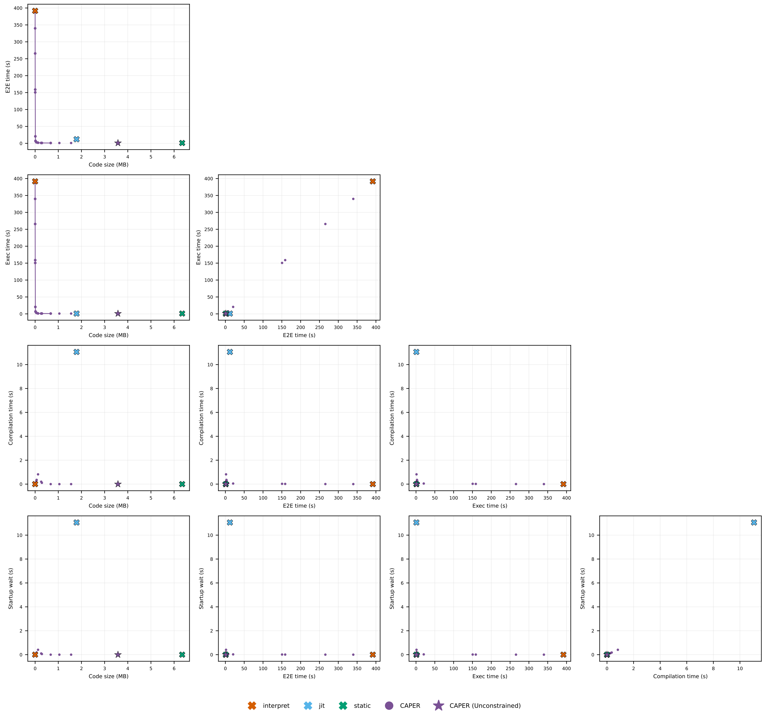
SQLite · subquery-correlated: pairwise metric trade-offs
