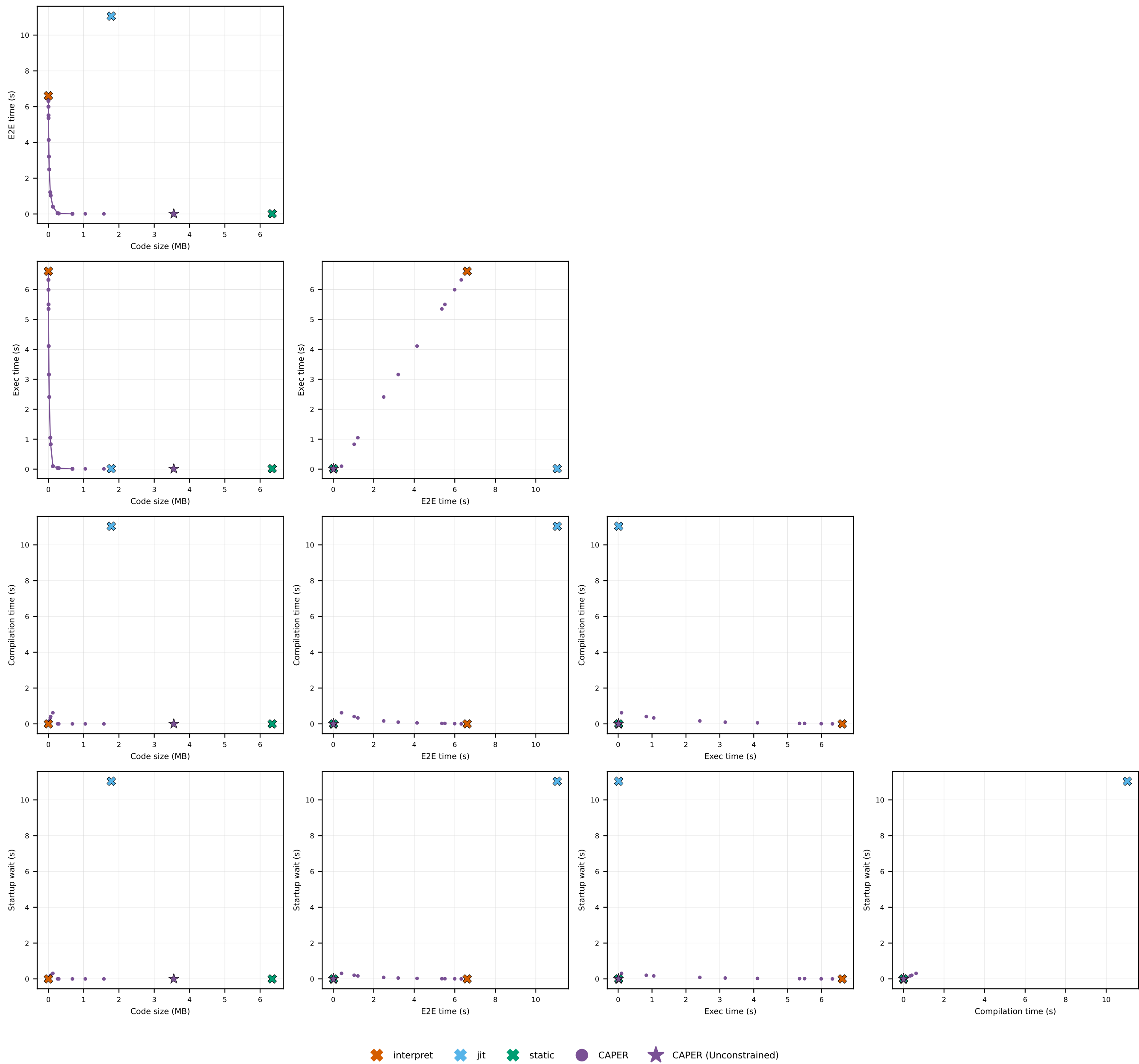
SQLite · with-recursive-cte: pairwise metric trade-offs
