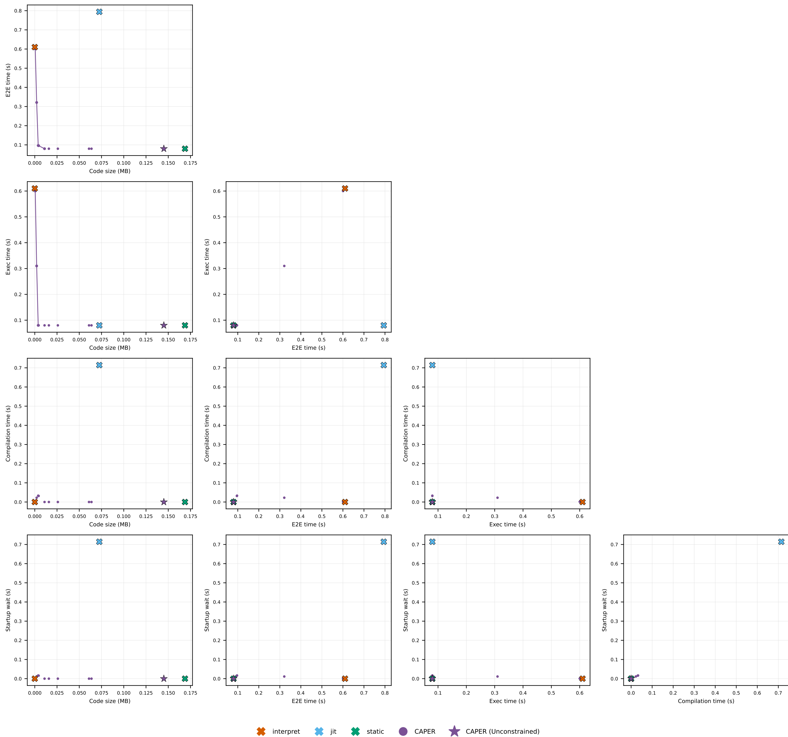
trisolv · trisolv: pairwise metric trade-offs
