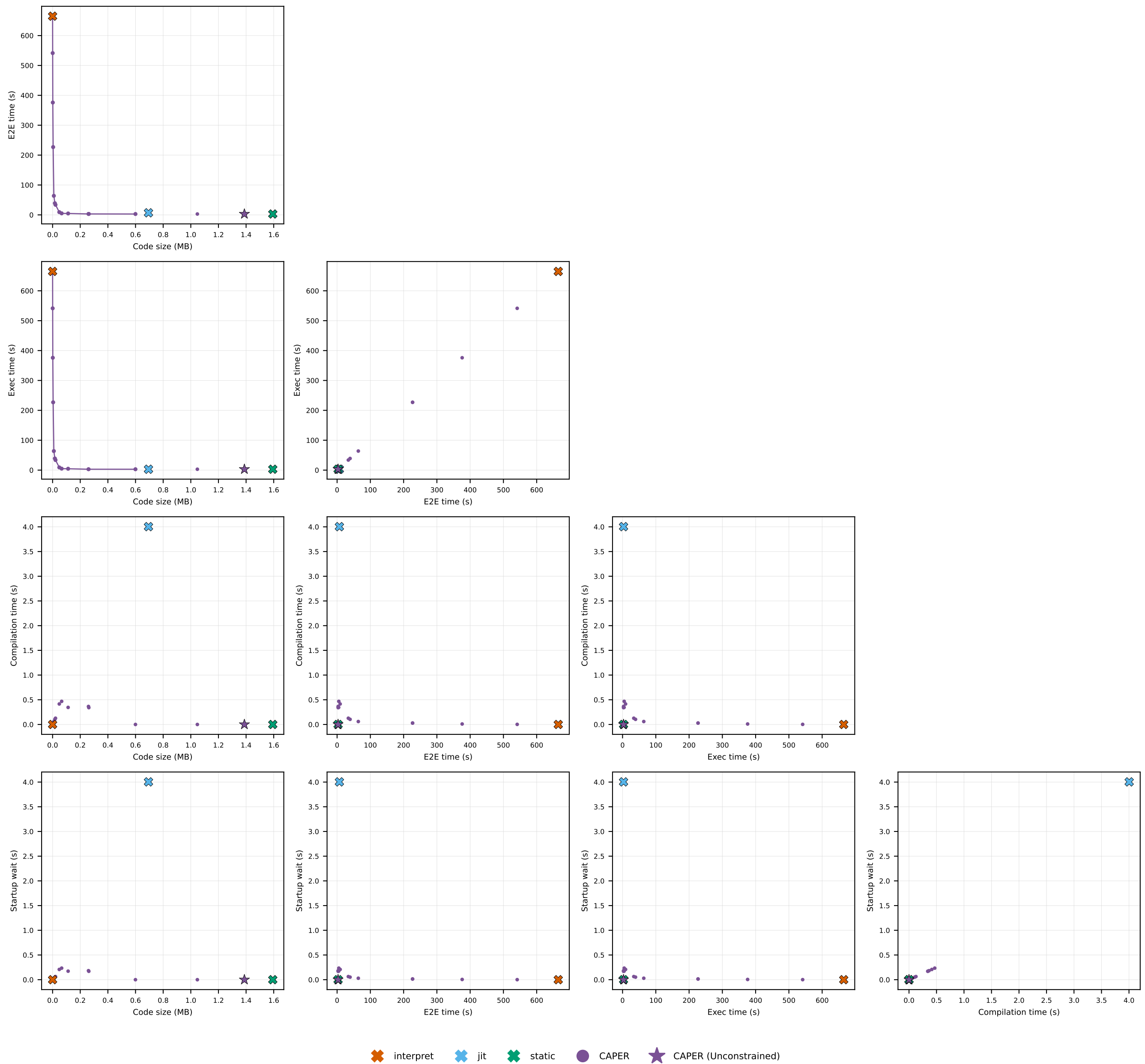
tsf · tsf: pairwise metric trade-offs
