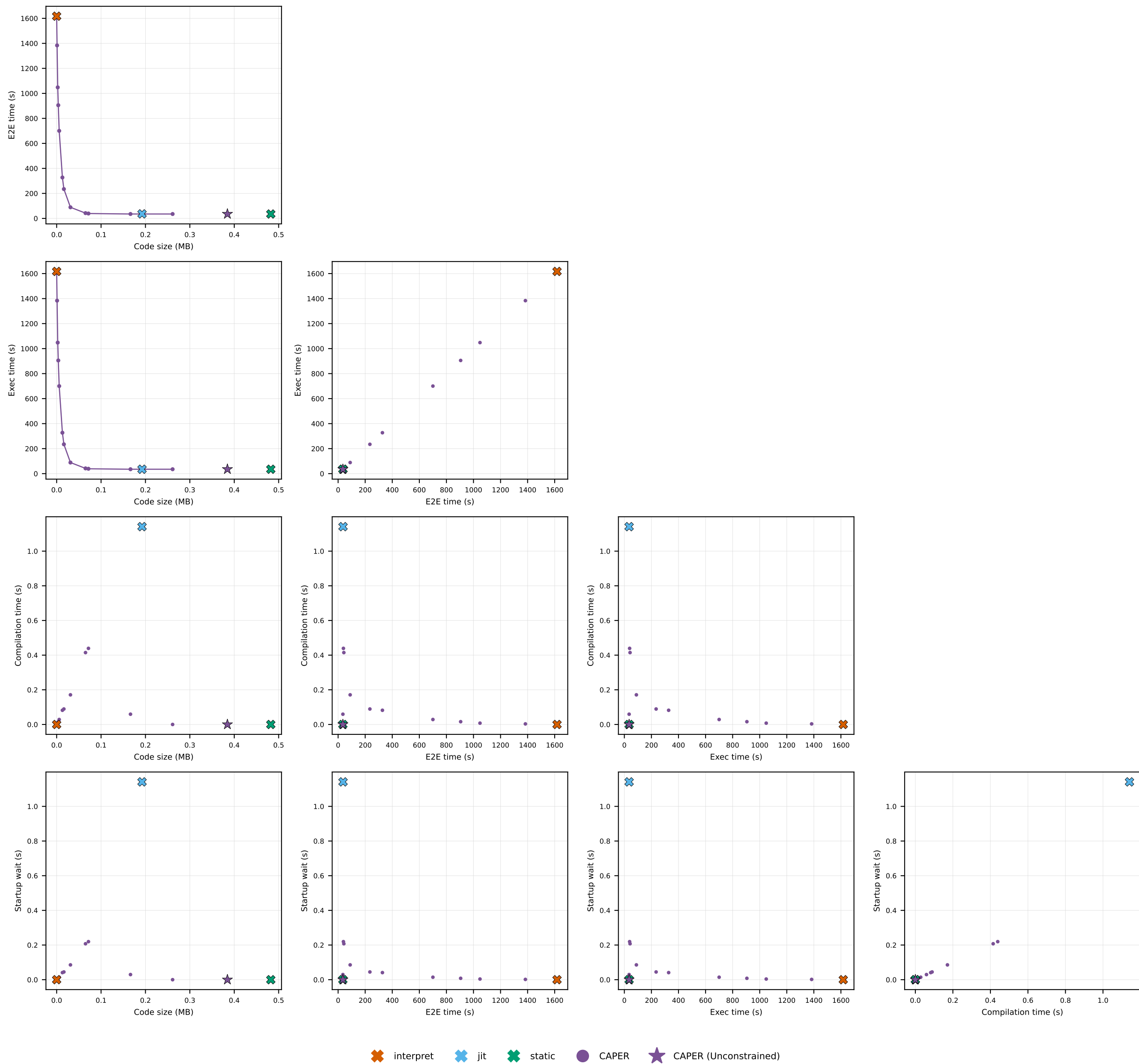
whitedb · whitedb: pairwise metric trade-offs
