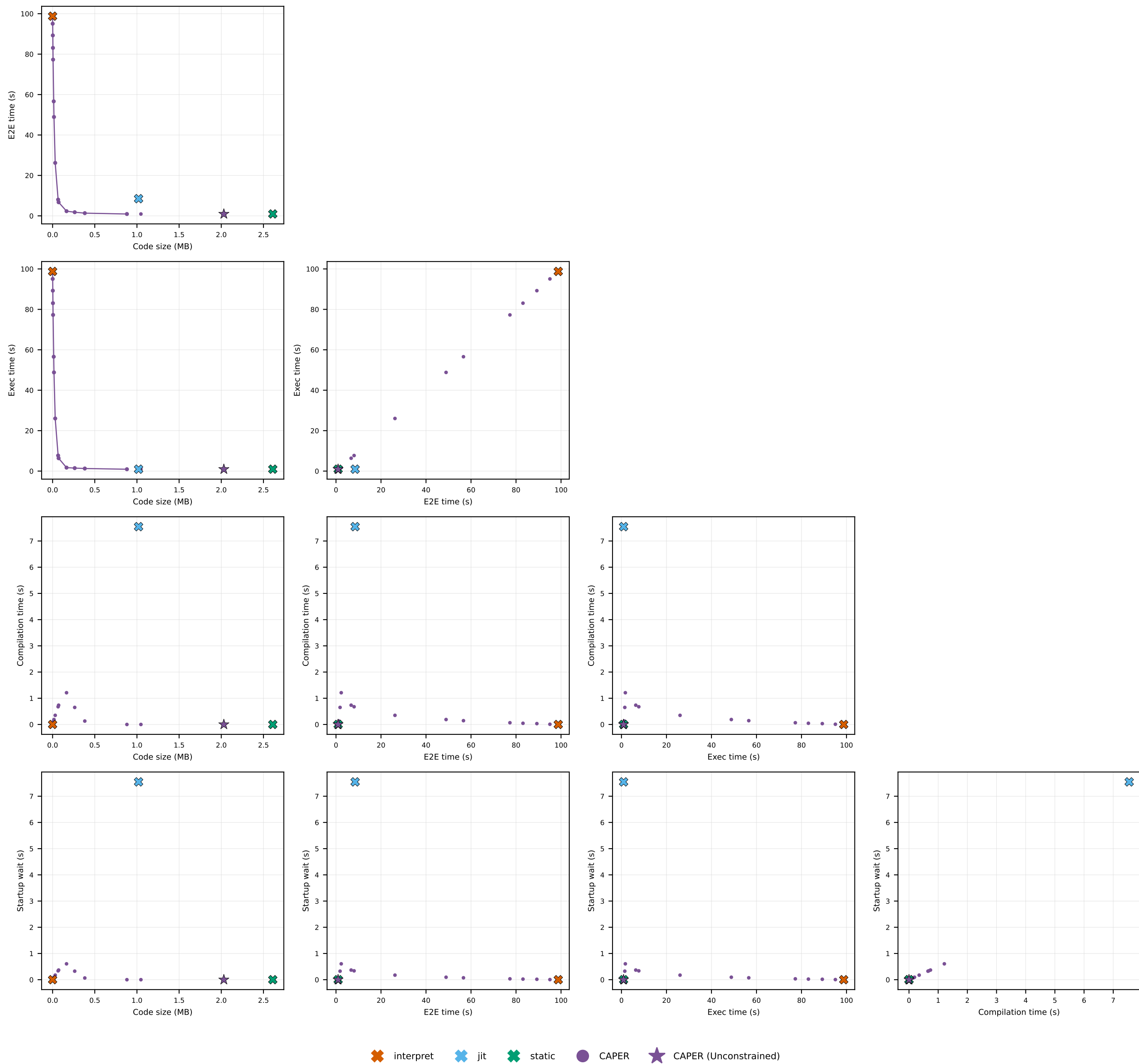
x264 · x264: pairwise metric trade-offs
