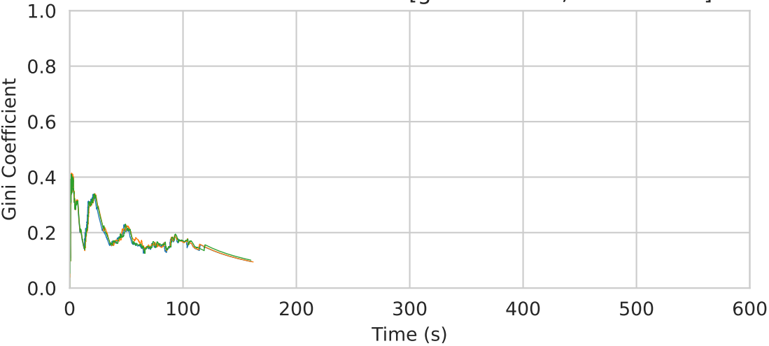
Gini Coefficient Over Time [global=1750, local=2250]
