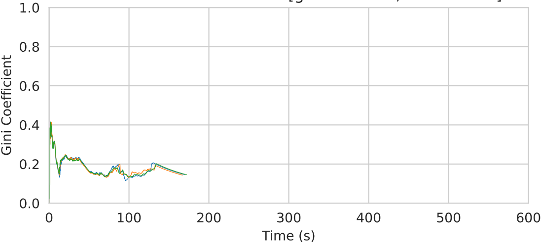
Gini Coefficient Over Time [global=2000, local=1000]
