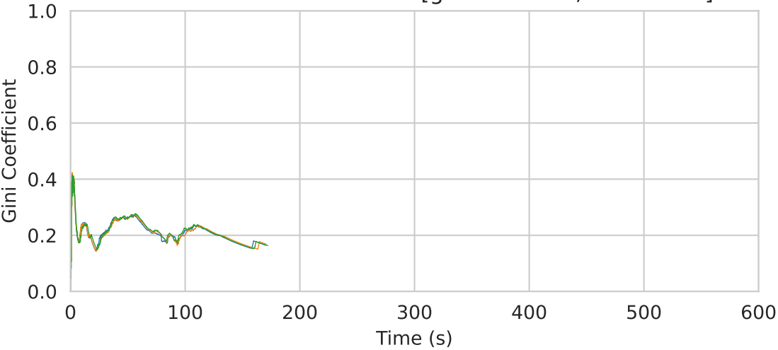
Gini Coefficient Over Time [global=2000, local=500]
