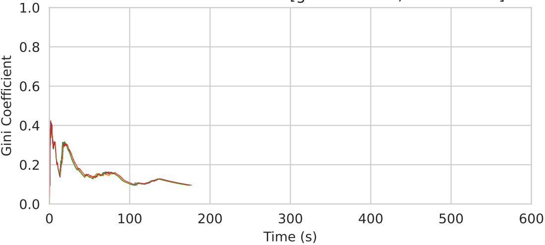
Gini Coefficient Over Time [global=2250, local=1250]
