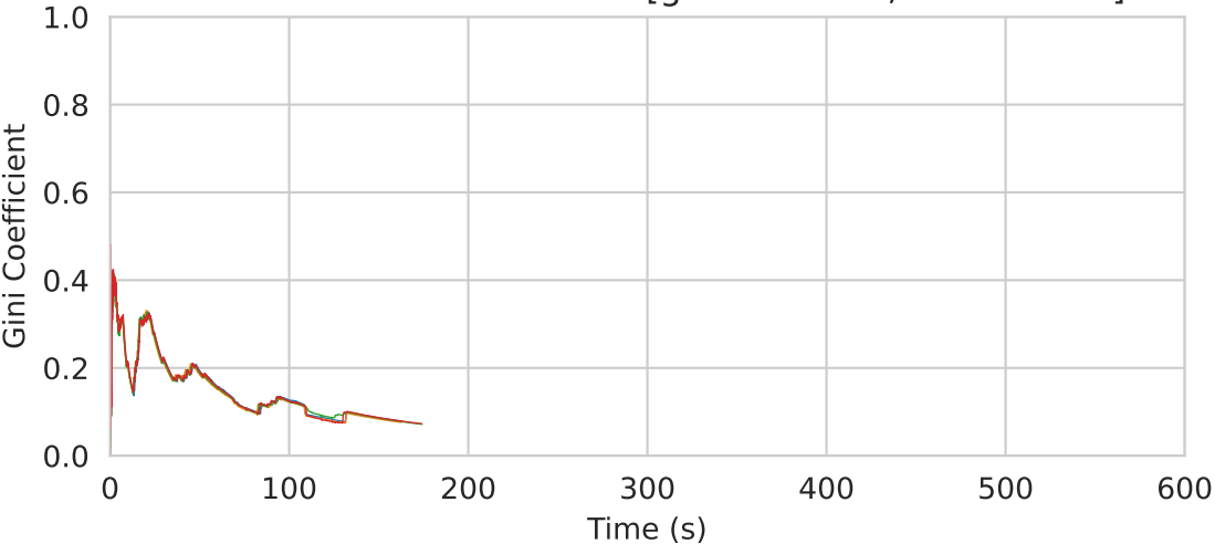
Gini Coefficient Over Time [global=2250, local=2000]
