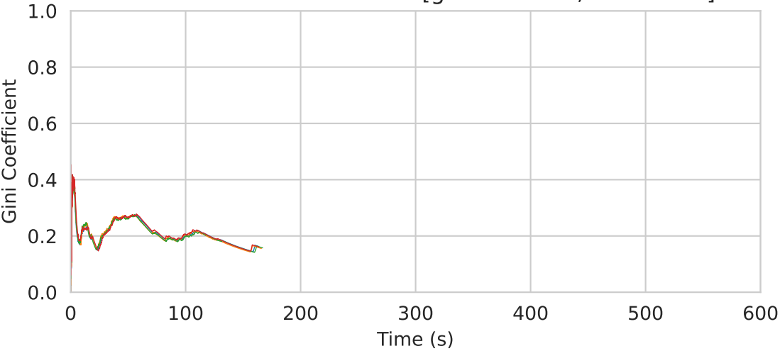
Gini Coefficient Over Time [global=2250, local=500]
