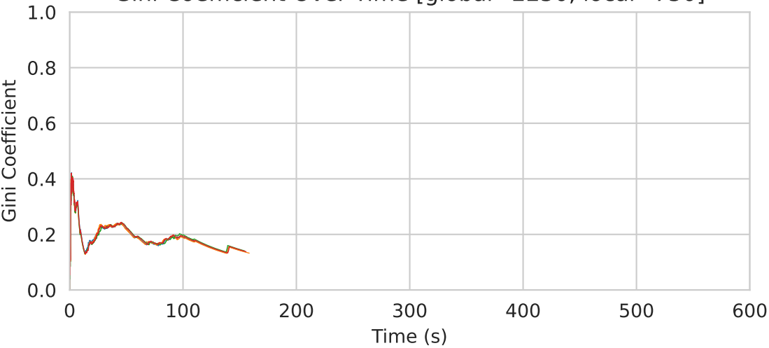
Gini Coefficient Over Time [global=2250, local=750]
