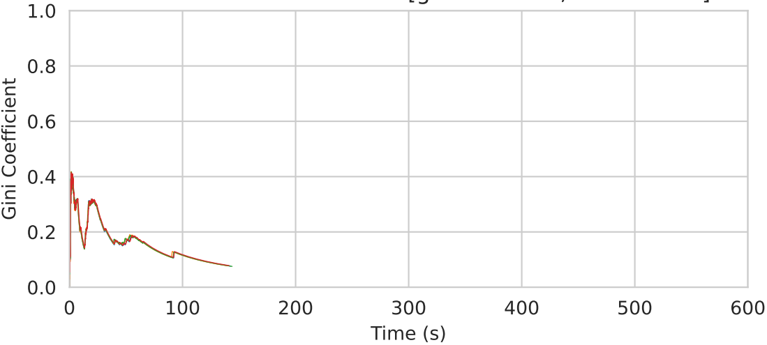
Gini Coefficient Over Time [global=2500, local=1750]
