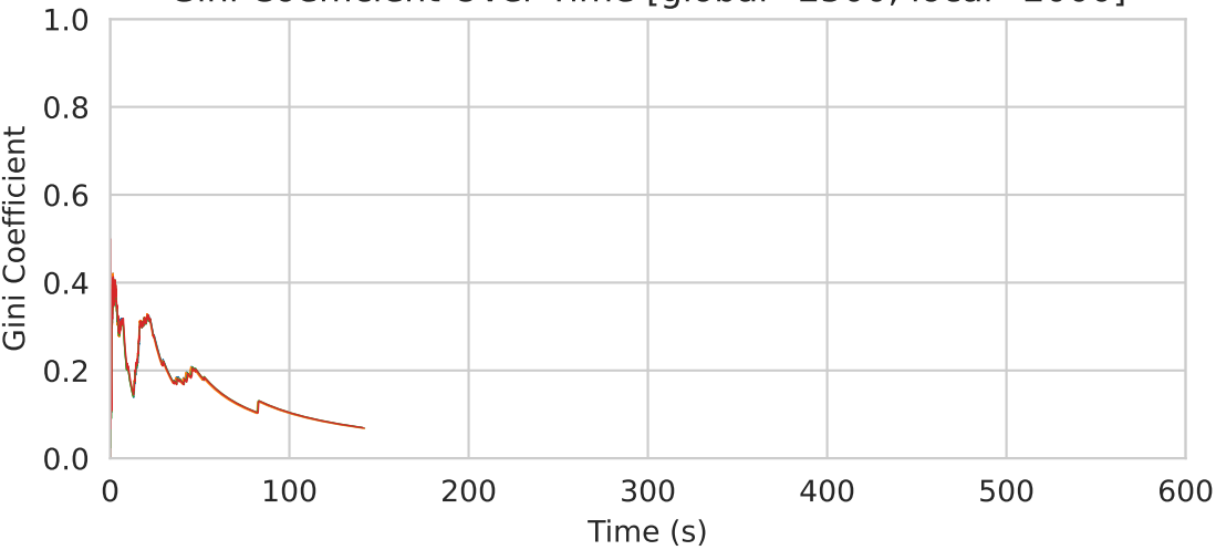
Gini Coefficient Over Time [global=2500, local=2000]
