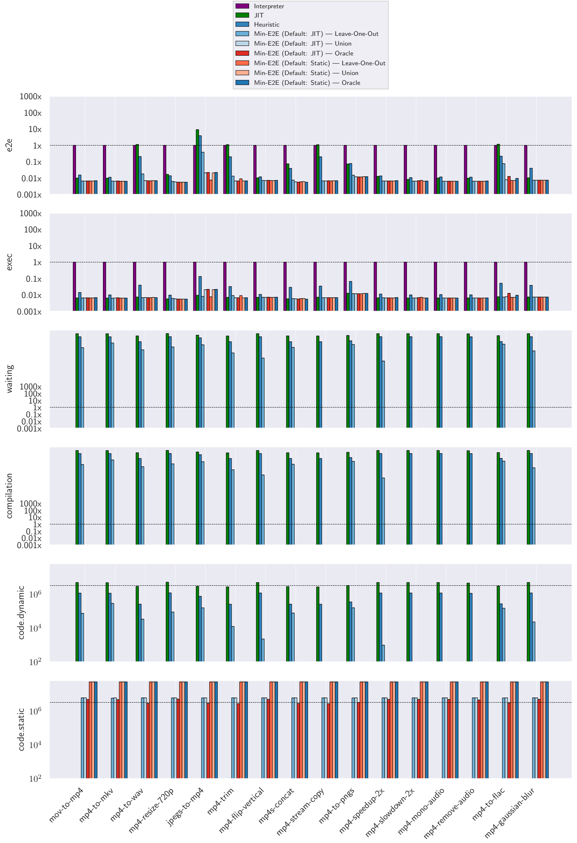
ffmpeg Compilation Plans Comparison
