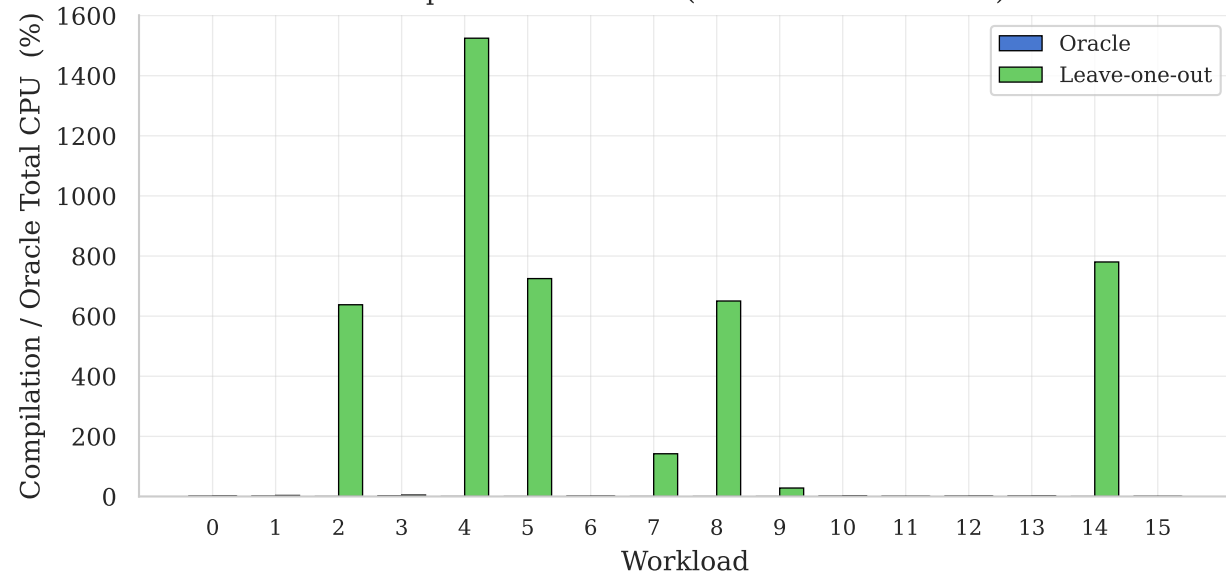
Compilation Overhead (relative to oracle CPU)
