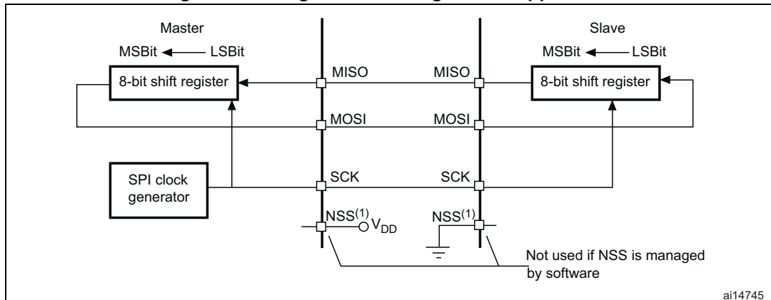
Figure 193. Single master/ single slave application
