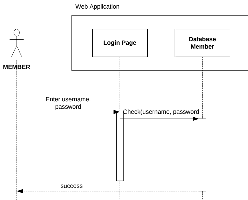
រូបភាព 6.5 Sequence diagram (Login)
