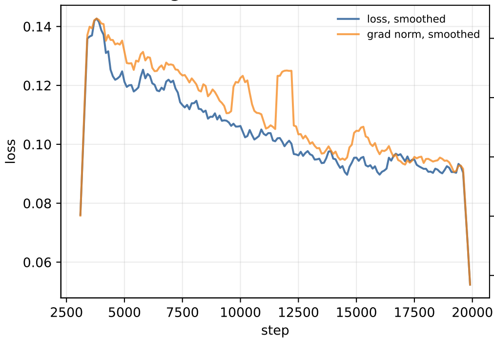
LoRA training curve
