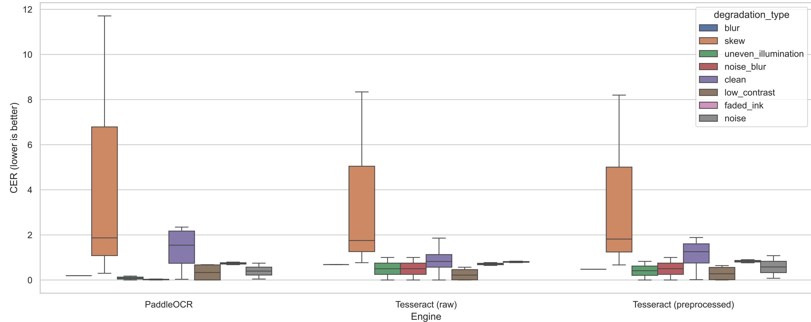
CER Comparison by Degradation Type (Normalized Mode)
