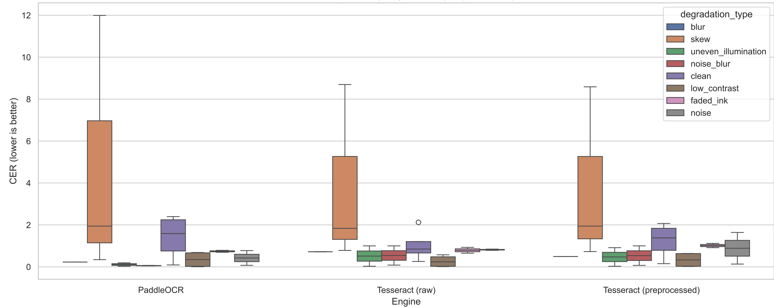
CER Comparison by Degradation Type (Strict Mode)
