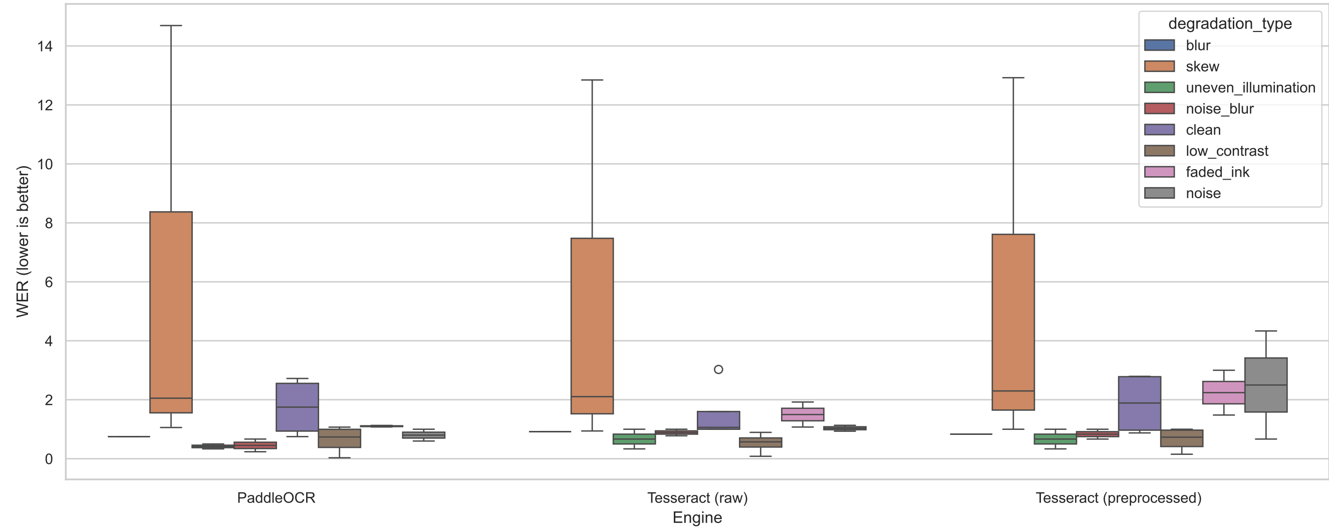
WER Comparison by Degradation Type (Strict Mode)
