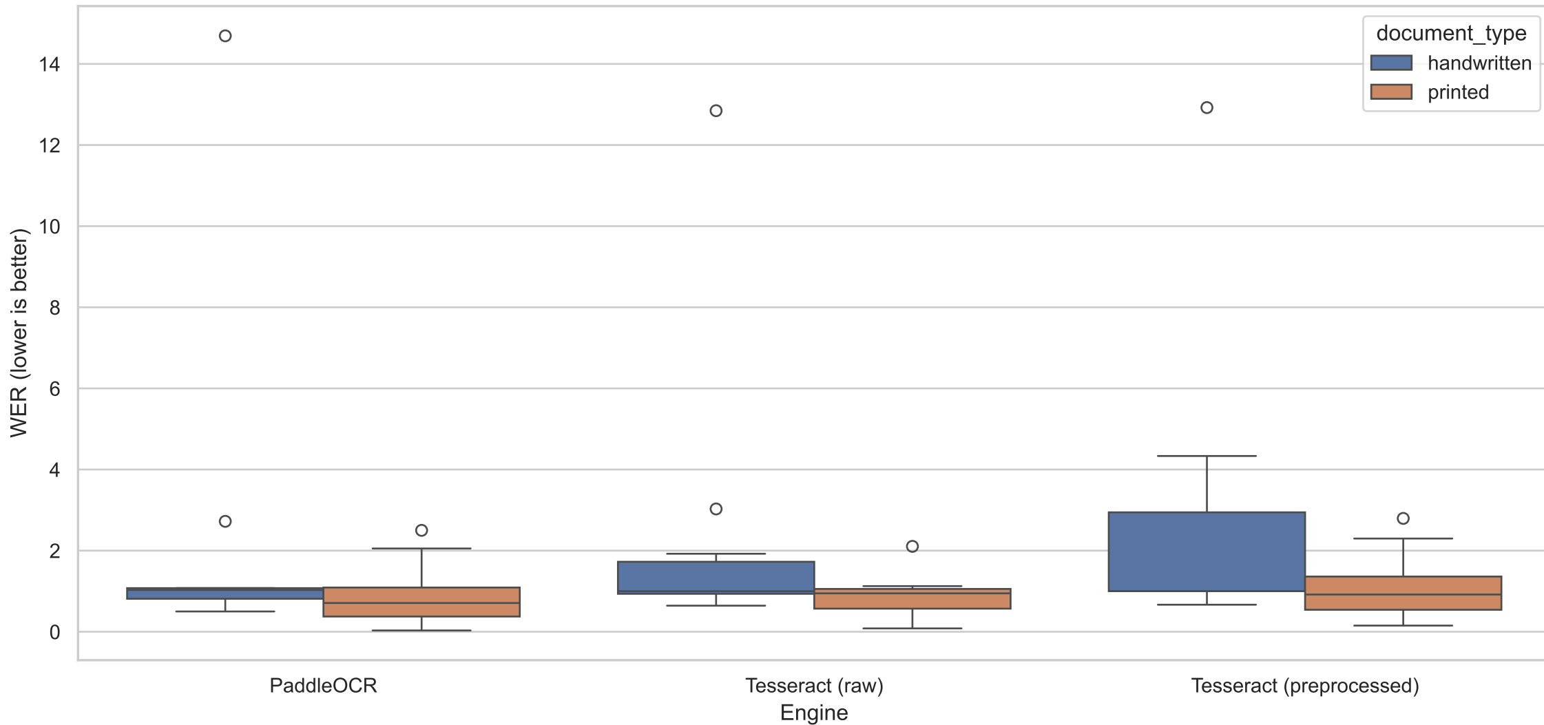
WER Comparison by Document Type (Strict Mode)
