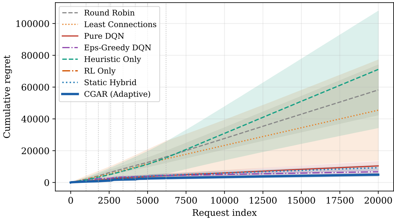
Cumulative Regret with 95% Confidence Interval
