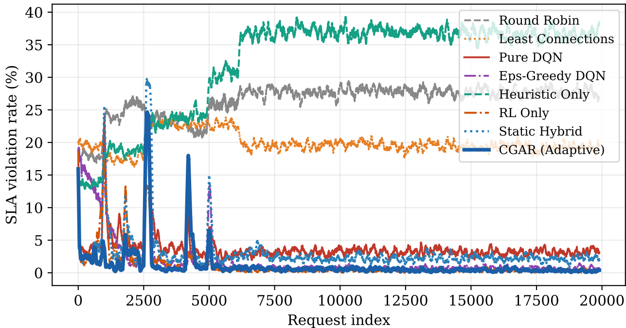
Rolling SLA Violation Rate
