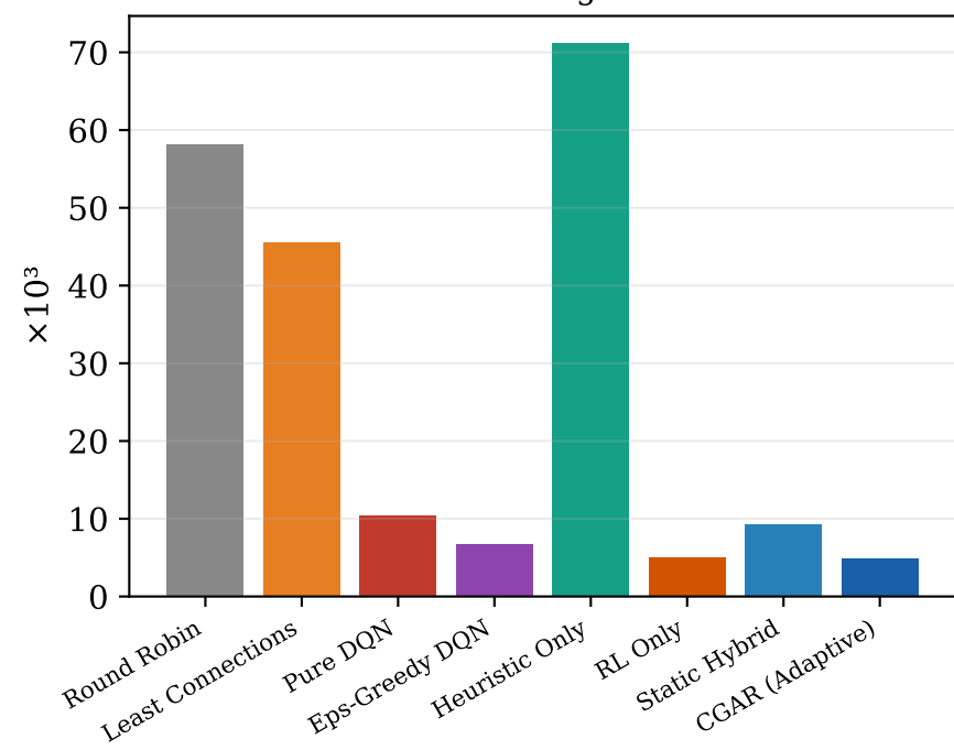
Total Regret
