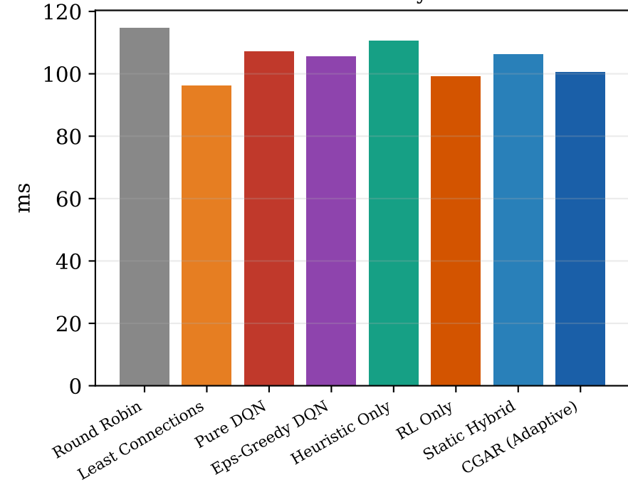
P99 Latency
