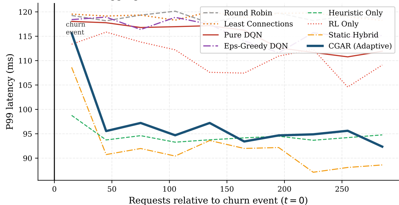
P99 Latency Around Backend Pool Churn Events (aggregated across all churn events and seeds)
