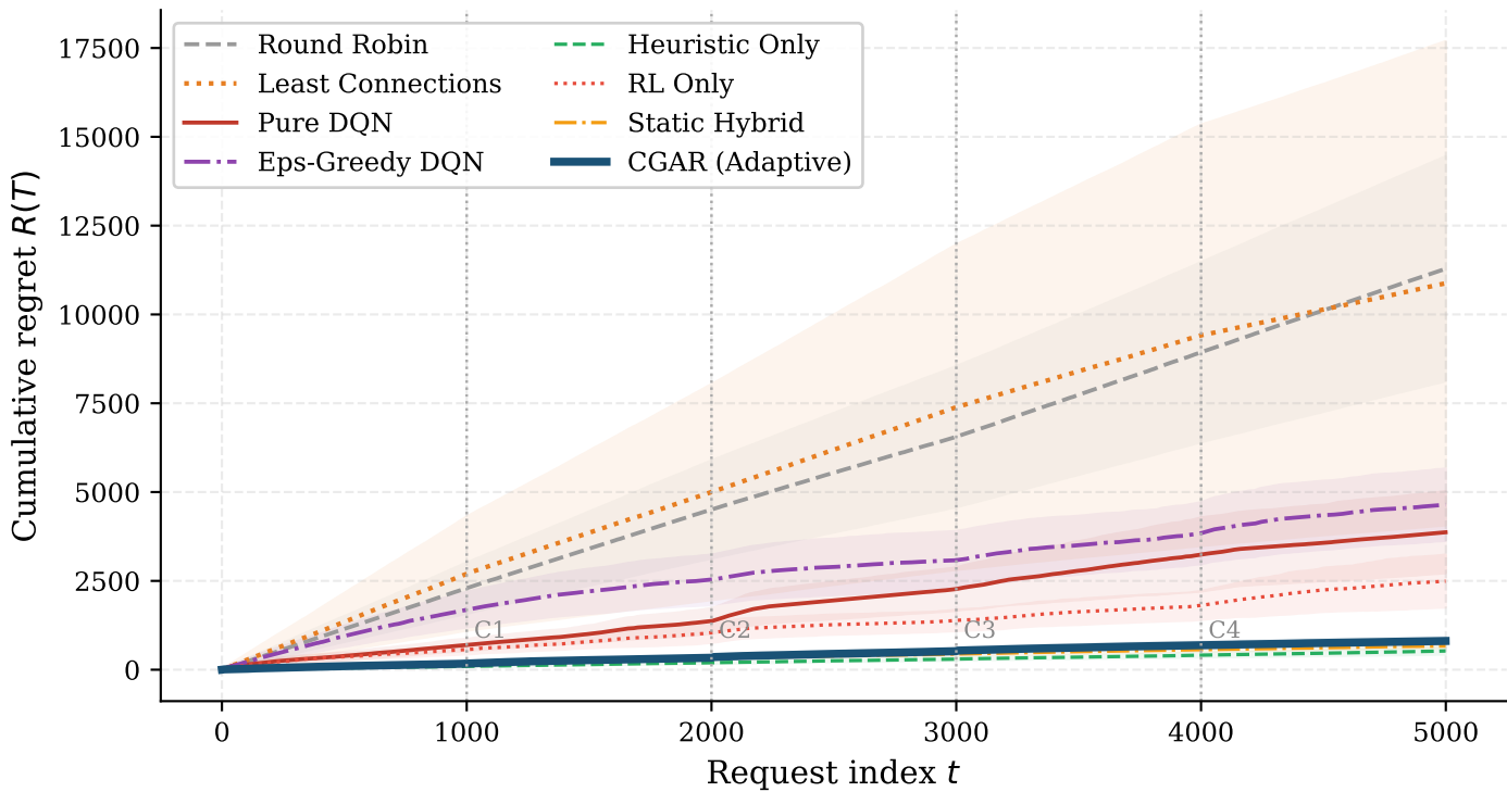
Cumulative Regret vs. Request Index (mean \pm 95% CI, 20 seeds; C1-C4 = churn events)
