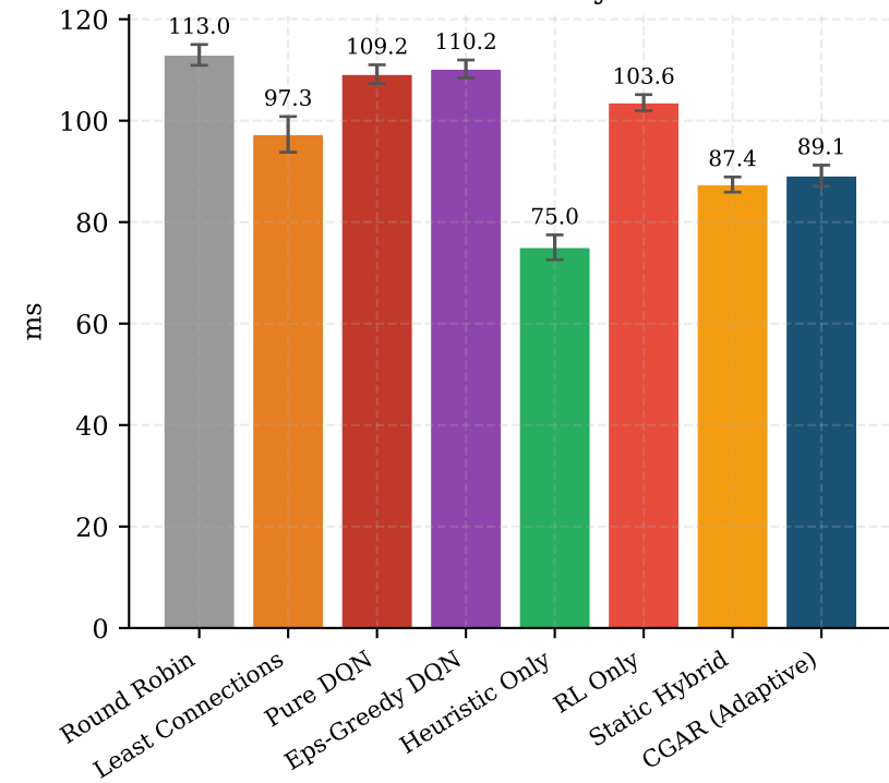
P99 Latency
