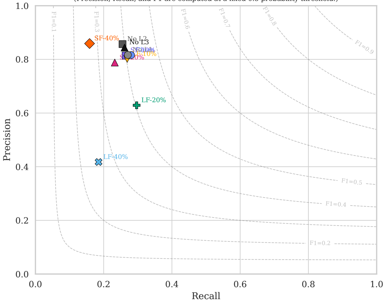
Figure 8: Precision vs. Recall (Round 50) The grey dashed contours represent constant F1 values. (Precision, Recall, and F1 are computed at a fixed 0.5 probability threshold.)
