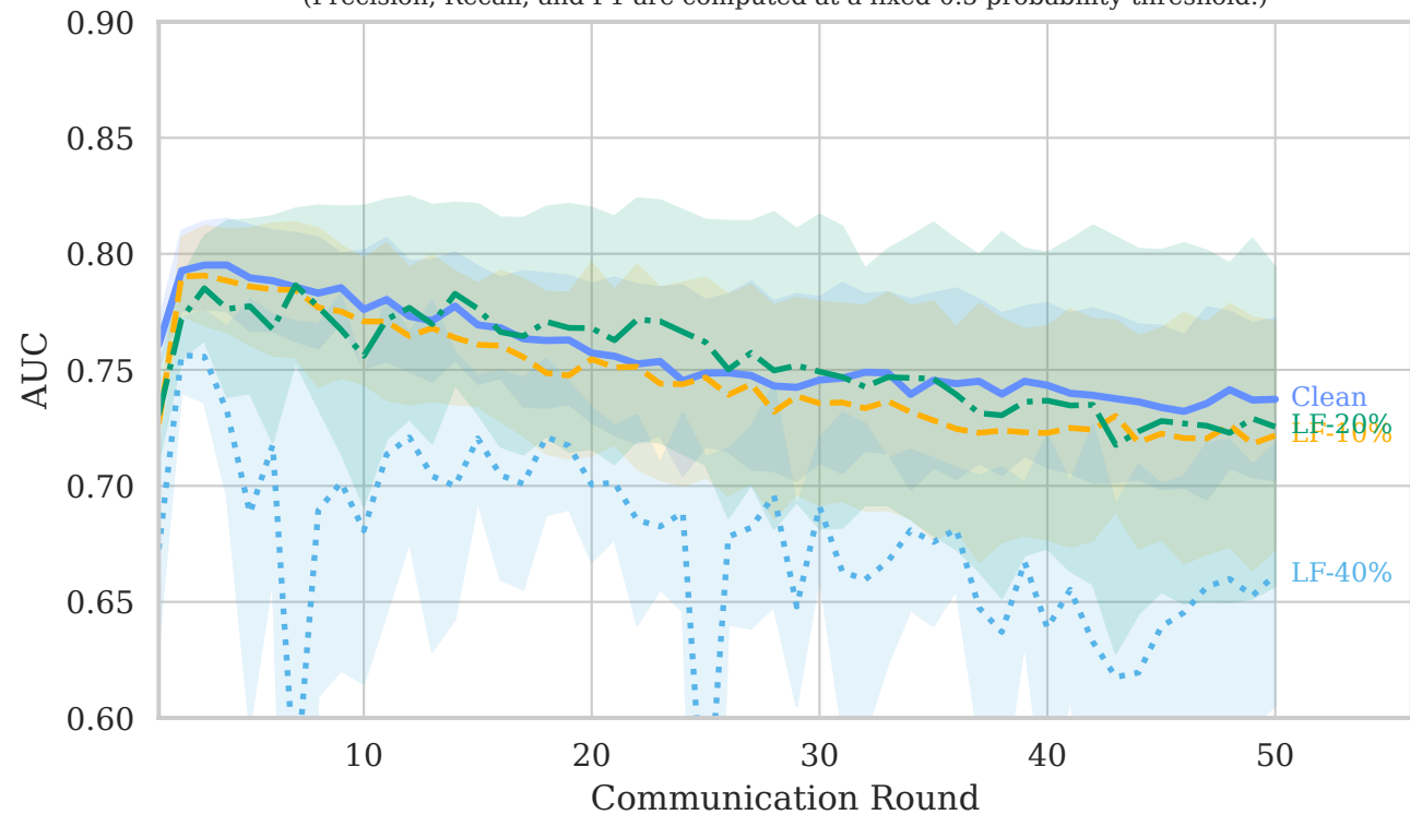
Figure 3: AUC Under Label-Flip Attacks (Precision, Recall, and F1 are computed at a fixed 0.5 probability threshold.)
