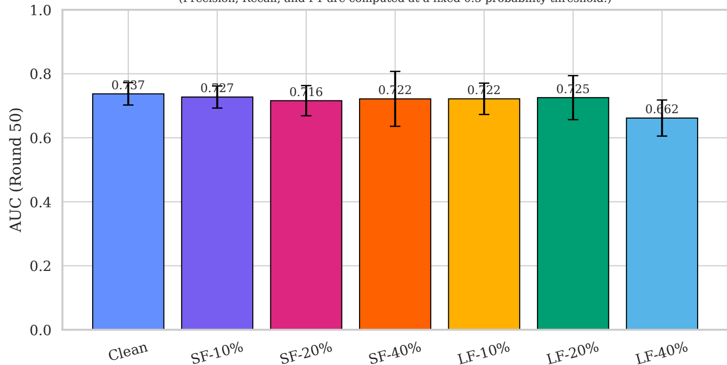
Figure 4: Final-Round AUC by Attack Scenario (Precision, Recall, and F1 are computed at a fixed 0.5 probability threshold.)
