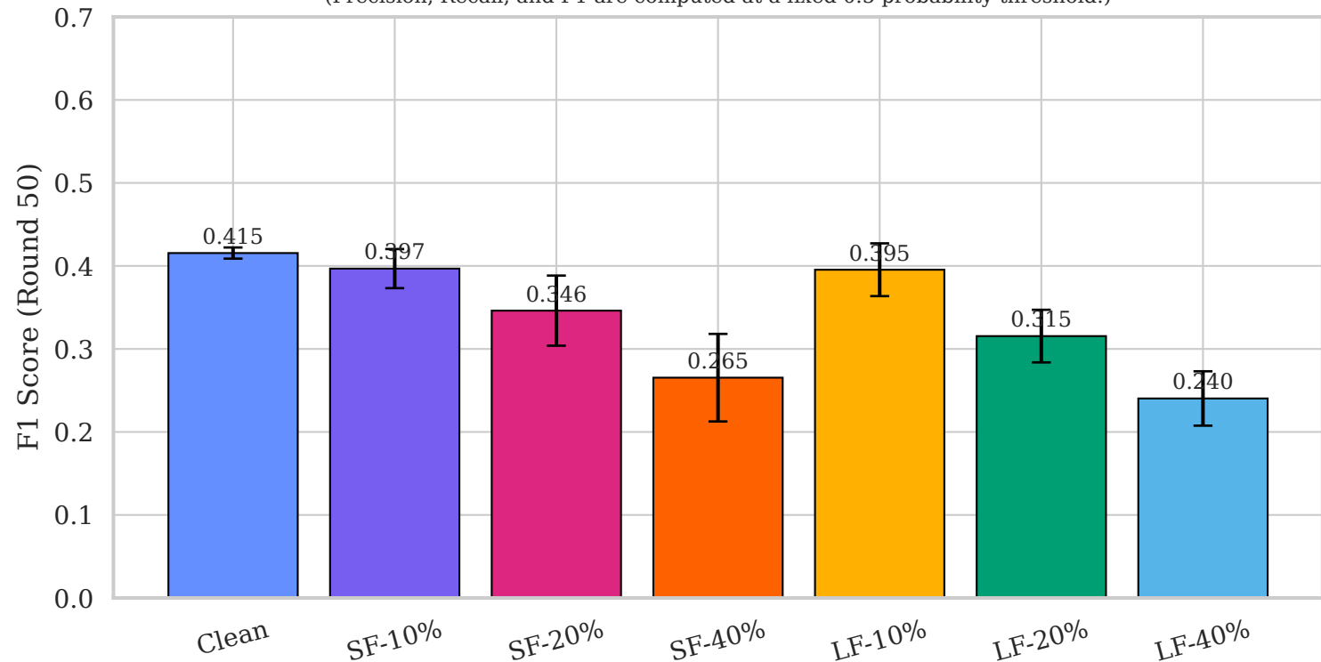
Figure 5: Final-Round F1 by Attack Scenario (Precision, Recall, and F1 are computed at a fixed 0.5 probability threshold.)
