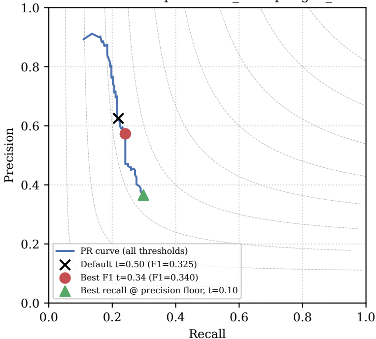
Threshold sweep — Clean_SweepRegen_r50
