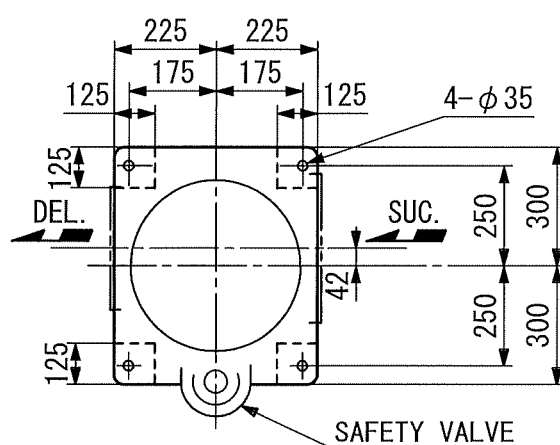
A-A ARROW VIEW
