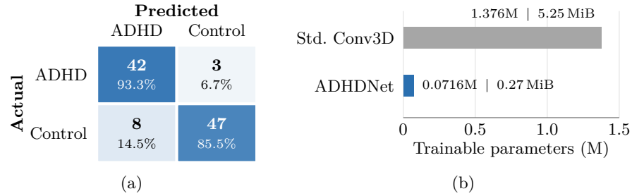
Fig. 2. (a) Confusion matrix of ADHDNet on the held-out validation set ( n = 100 ); cell shading and percentages are normalized by the actual class. (b) Trainable parameters of ADHDNet and the standard Conv3D multimodal comparator, a 94.8% reduction; labels give the corresponding FP32 weight storage (parameters \times 4 bytes), not runtime memory usage.
