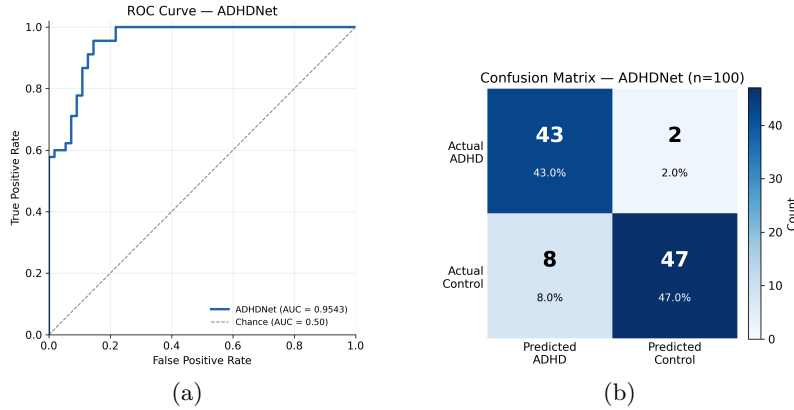
Fig. 2. Held-out validation results ( n = 100 ): (a) ROC curve ( \text{AUC} = 0.9543 ); (b) confusion matrix at threshold 0.5.
