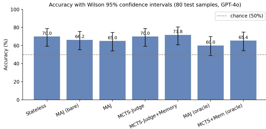
Figure 1 – Per-mode accuracy with Wilson 95% confidence intervals on the leakage-free, audited test set. The error bars of every mode overlap with those of the stateless baseline.
