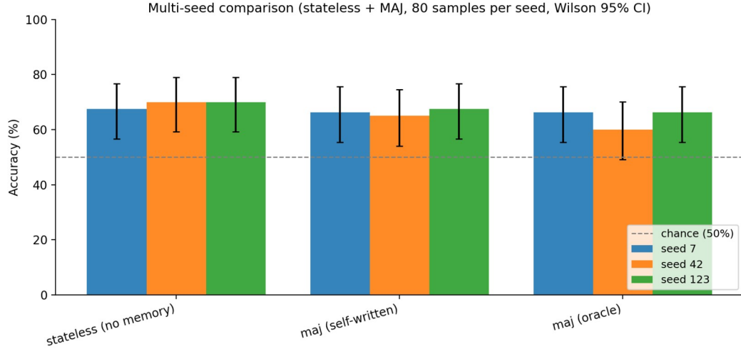
Figure 6 – Cross-seed comparison of the stateless and memory-augmented modes over three random splits, with Wilson 95% confidence intervals. The cross-seed spread of each mode is wider than the gap between modes.
