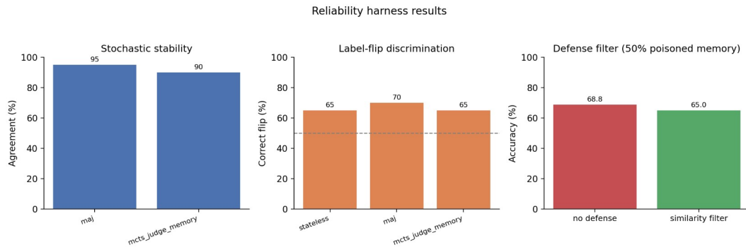
Figure 8 – Reliability harness results: stochastic stability, label-flip discrimination, and the defense filter under 50% poisoned memory.
