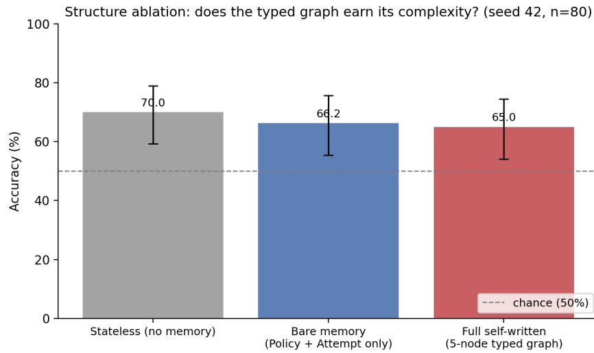
Figure 5 – Structure ablation: accuracy of the stateless baseline, a bare Policy-plus-Attempt memory, and the full five-node typed graph, with Wilson 95% confidence intervals. The three intervals overlap.
