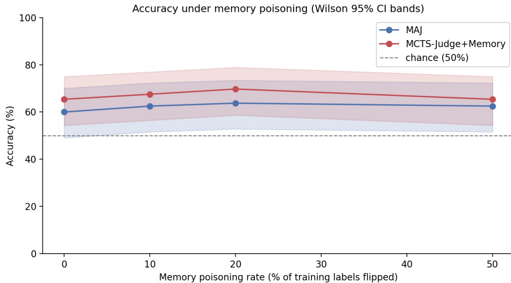
Figure 7 – Accuracy as a function of the memory poisoning rate, under the corrected, audited harness, with Wilson 95% confidence interval bands. Neither mode shows a significant downward trend as the corruption rate rises.
