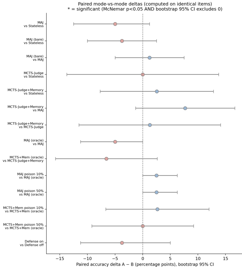
Figure 2 – Paired accuracy differences between modes, computed on identical items, with bootstrap 95% confidence intervals. An interval crossing the dashed zero line indicates a non-significant difference; all clean-memory comparisons do so.
