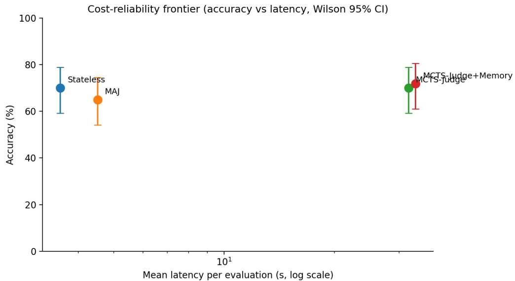
Figure 9 – Cost-reliability frontier: accuracy against mean latency per evaluation (logarithmic scale), with Wilson 95% confidence intervals. The MCTS modes cost roughly an order of magnitude more latency without a corresponding accuracy gain.
