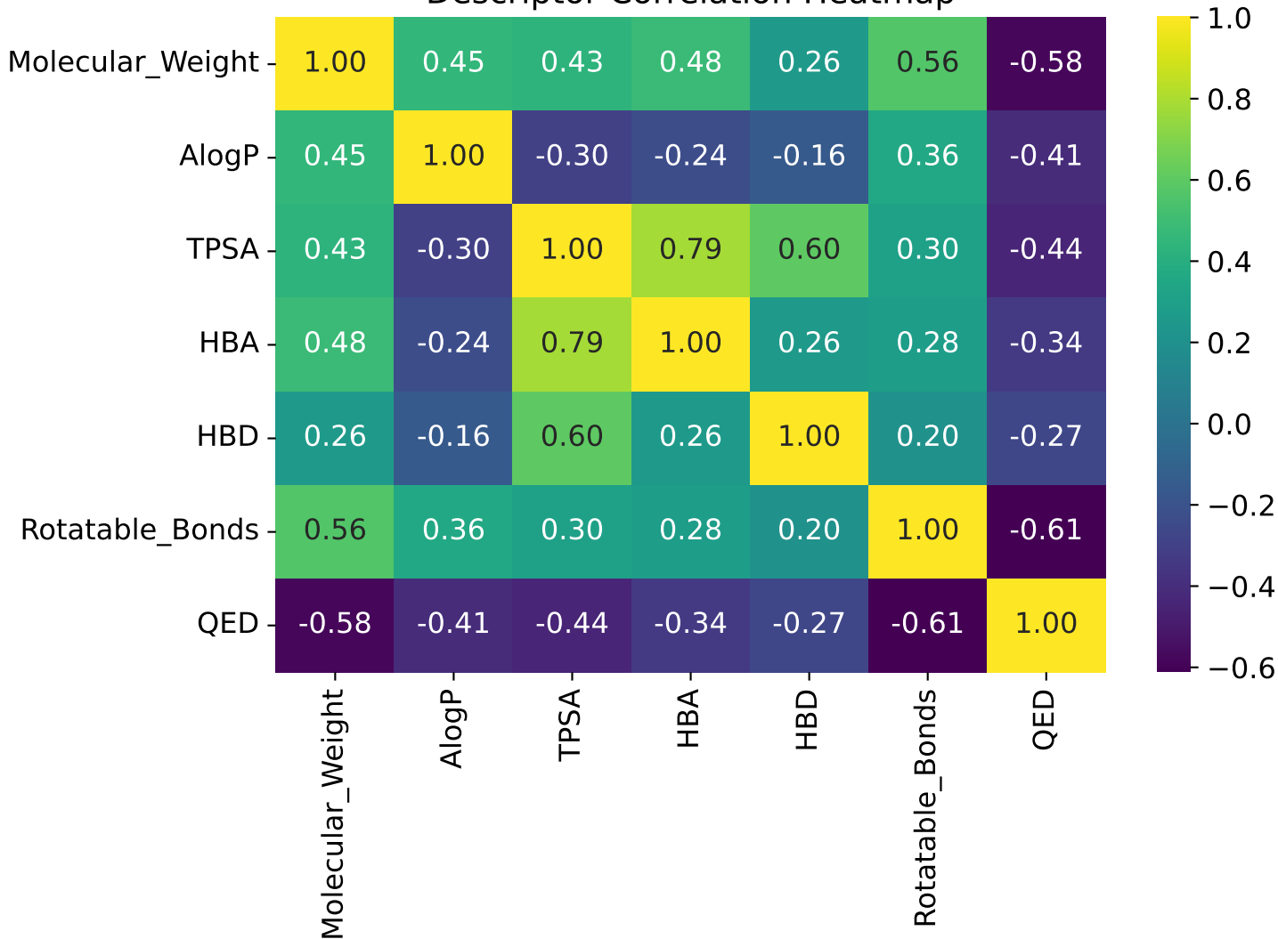
Descriptor Correlation Heatmap
