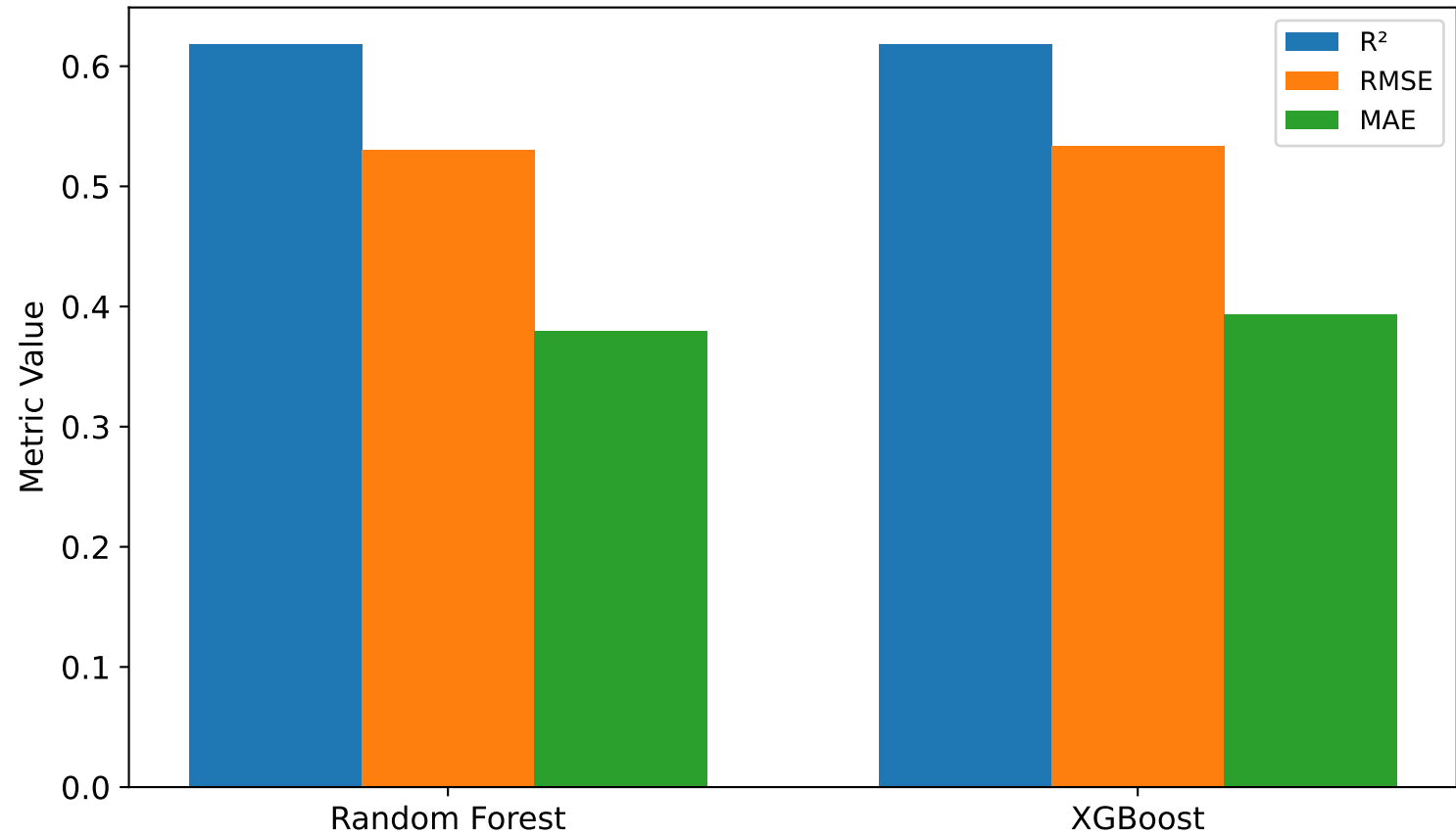
Model Comparison Summary
