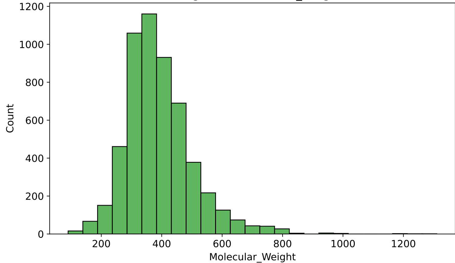
Histogram of Molecular_Weight
